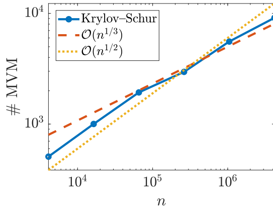
FIG. 3. The number of matrix-vector multiplications (MVMs) needed to estimate the leftmost eigenvalue with the Krylov-Schur method, as a function of the number of image pixels n .
