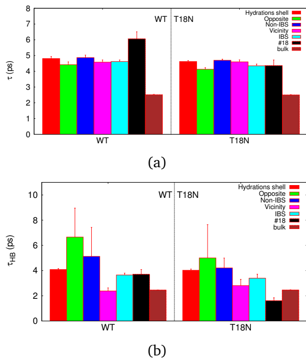
Figure 4: a) Water reorientation time, b) protein water H-bond lifetimes of hydration water for the WT and T18N fully hydrated systems at room temperature. Color coding as in Fig. 1.
