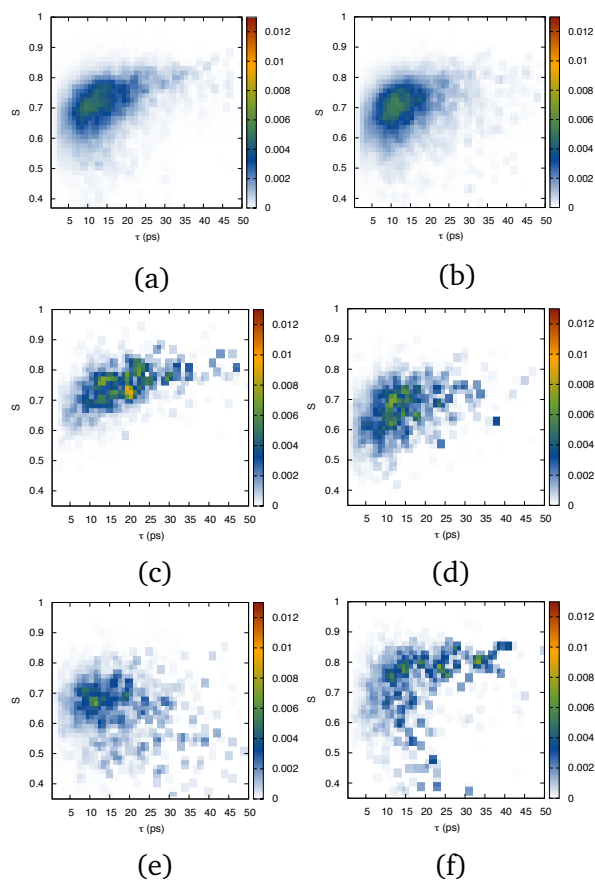
Figure 7: Structural parameter S as a function of water reorientation decay time for selected residues of a) IBS (WT), b) IBS (T18N), c) THR-18 (WT), d) ASN-18 (T18N), e) ARG-39 (WT/vicinity), f) ALA-48 (WT/vicinity) at 270 K for the fully hydrated systems.
