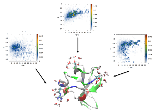
Figure 12: Signal of anti-correlation of tetrahedral structure of water ( S ) and its OH reorientation decay time ( \tau ) for selected amino-acids of the Ice Binding Site vicinity (left and right) and positive correlation between the tetrahedral structure of water ( S ) and its OH reorientation decay time ( \tau ) of the Ice Binding Site central amino-acid (middle).
