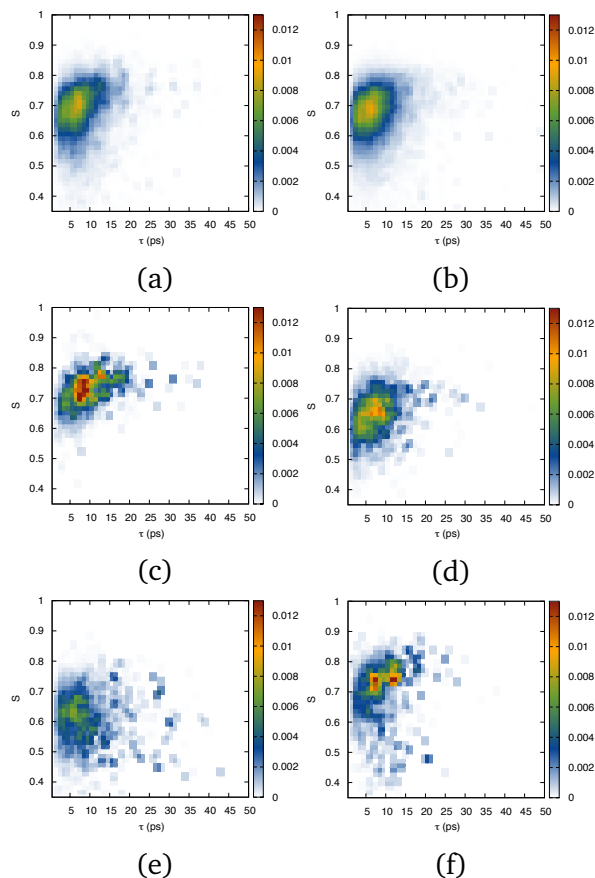
Figure 6: Structural parameter S as a function of water reorientation decay time for selected residues of a) IBS (WT), b) IBS (T18N), c) THR-18 (WT), d) ASN-18 (T18N), e) ARG-39 (WT/vicinity), f) ALA-48 (WT/vicinity) at 298 K for the fully hydrated systems.
