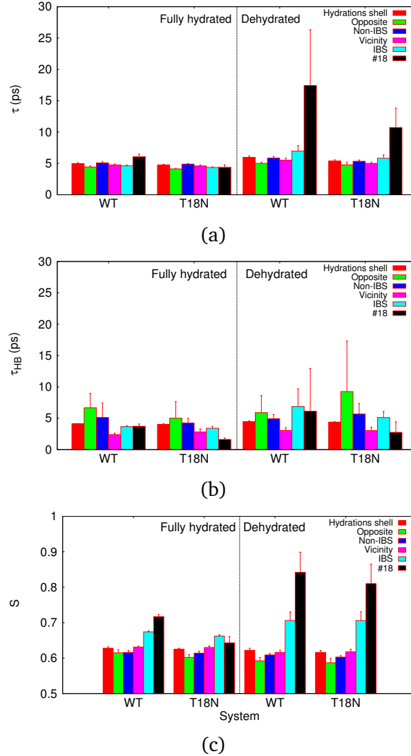
Figure 10: a) Water reorientation time, b) protein water H-bond lifetimes, and c) structural parameter S of hydration water for fully hydrated WT and T18N systems, and for dehydrated WT and T18N systems at 298 K.
