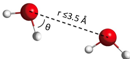
Figure 2: Definition of the \theta angle.
