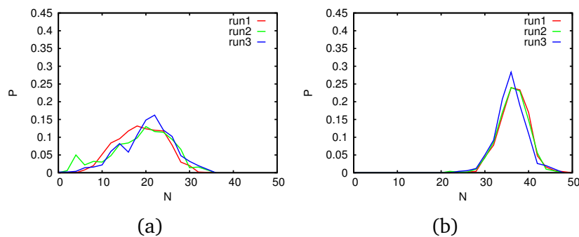
Figure 11: Distribution of number of water molecules within 0.65 nm of THR-18 and ASN-18 for a) WT slab geometry at 298 K and b) T18N slab geometry respectively at 298 K. Hydration for different radii of 0.45 nm and 0.55 nm are reported in Figure S54. Note that the THR-18 is less hydrated than ASN-18 for all different radii used.
