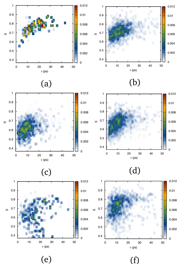
Figure 8: Structural parameter S as a function of water reorientation decay time for residue 18 for a) THR-18 (WT) H-bonded, b) THR-18 (WT) non H-bonded, c) ASN-18 (T18N) H-bonded, d) ASN-18 (T18N) non H-bonded, e) ALA-48 (WT) H-bonded, f) ALA-48 (WT) non H-bonded, for the fully hydrated systems at 270 K.
