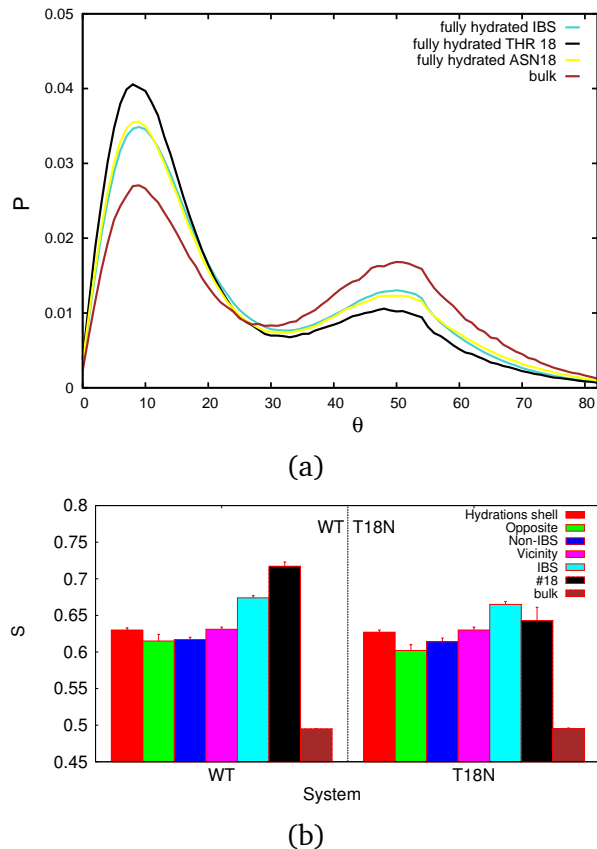
Figure 5: OOH angle distribution of water pairs solvating the wild fully hydrated system IBS (cyan), THR-18 of the WT fully hydrated system (black), ASN-18 of the T18N fully hydrated system (yellow), of the bulk water (brown). b) Structure order parameter of water ( S ), for the different parts of the protein. All the above systems are in room temperature. Color coding as in Fig. 1.
