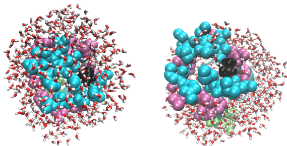
Figure 9: Starting frame of dehydrated NVT system (left) and a dehydrated protein at a frame after 100 ns (right). Protein color coding as in Fig. 1.
