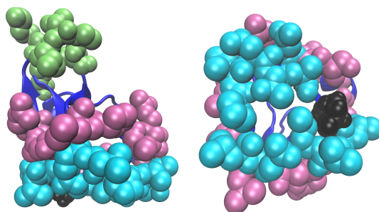
Figure 1: Partitioning of the protein into three distinct areas. The area IBS (denoted by cyan), vicinity (denoted by magenta) and opposite (denoted by green). THR-18 is denoted by black.
