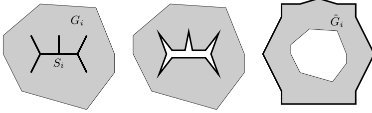
Figure 3: The process of cutting open the graph G_i along the tree S_i . Adapted from [27] with permission.
