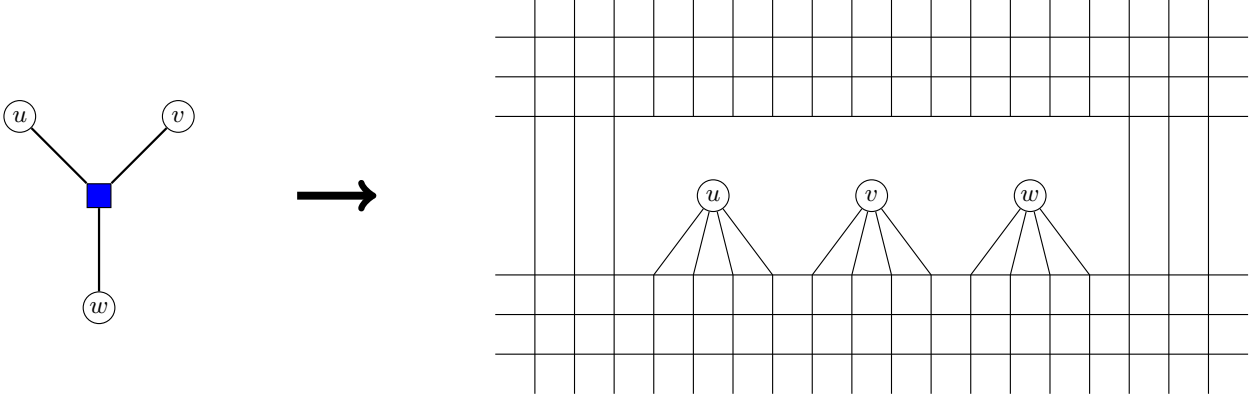
Figure 6: Embedding neighbors of a terminal (blue square) into a hole cut out in a large grid. Every neighbor of a terminal is connected to k + 1 vertices of the grid ( k + 1 = 4 in the figure).
