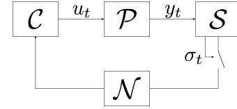
Fig. 1. Setup: an event-triggered controller consists of a controller \mathcal{C} and a scheduler \mathcal{S} ; \mathcal{N} represents the network, \mathcal{P} represents the plant, u_t , y_t , \sigma_t are the control input, output, and transmission decision, respectively, at time t . The scheduler sends measurement/estimation data to the controller.
