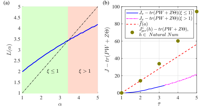
Fig. 2. (a) Result of the Monte Carlo simulations to find the range of \alpha satisfying the consistency condition of the ETC. (b) Trade-off curve between the performance and average inter-transmission time for the event-triggered and periodic control. Note that for the same integer average inter-transmission time, the ETC policy results in a performance cost significantly below than the performance cost of periodic control.
