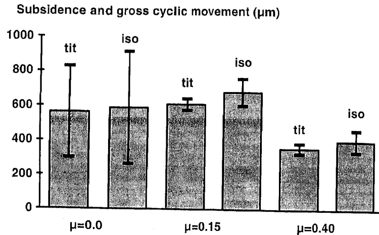
FIG. 3. Average subsidence of the stem tip (gray bar) and amplitude of gross cyclic movements ( \Sigma ) in the steady state for two values of the prosthetic Young's modulus (equivalent to titanium [tit] and isoelastic [iso]) and three values of the coefficient of friction ( \mu ) between bone and implant.
