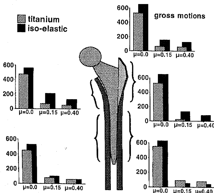
FIG. 4. Amplitudes of the cyclic interface motions along the interface in the steady state for two values of the prosthetic Young's modulus and three values of the coefficient of friction ( \mu ) between bone and implant.
