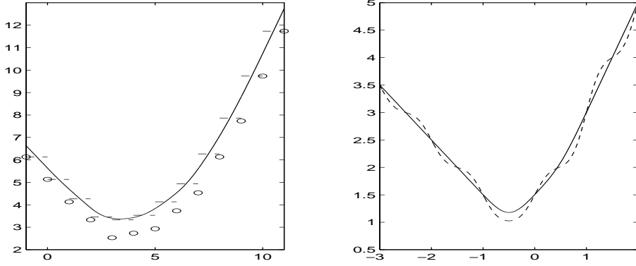
Figure 3.2: Approximations of the function Q ( q^+ = 1 , q^- = 2 ) by replacing the distribution F by the distribution f(s) = F(s + 1/2) - F(s - 1/2) , s \in \mathbb{R} . The function value in discontinuity points is depicted by \circ , the function Q by a dashed curve, and the approximation by a solid curve. Left: F is the discrete distribution on \{1, 3, 5, 7, 9\} with probabilities 1/15, 5/15, 3/15, 4/15, 2/15 , respectively. Right: F is the normal distribution with mean value 0 and variance 0.05.
