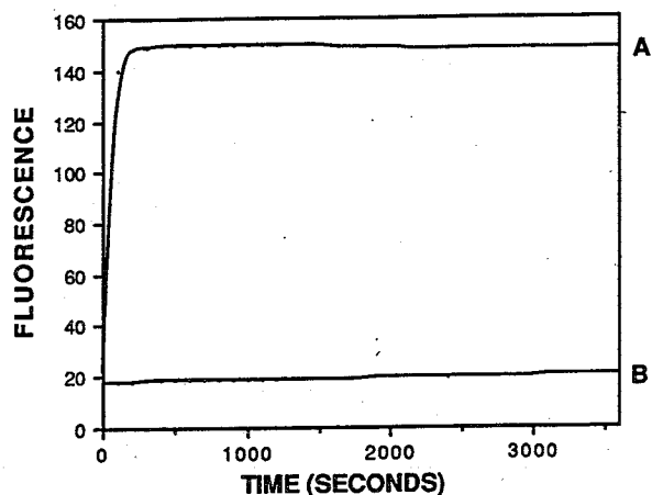
Figure 1. (A) Fluorescence vs time for addition of acetylcholinesterase ( 1.1 \times 10^{-8} M) to vesicles of I ( 6.5 \times 10^{-5} M) encapsulating II ( 2.2 \times 10^{-7} M) at pH = 6.8 and 30.0 °C. Excitation and emission wavelengths are 400 and 500 nm, respectively. The enzyme frees II and hydrolyzes it to a fluorescent product. (B) Base line obtained when no enzyme, or denatured enzyme, was added under equivalent conditions.
