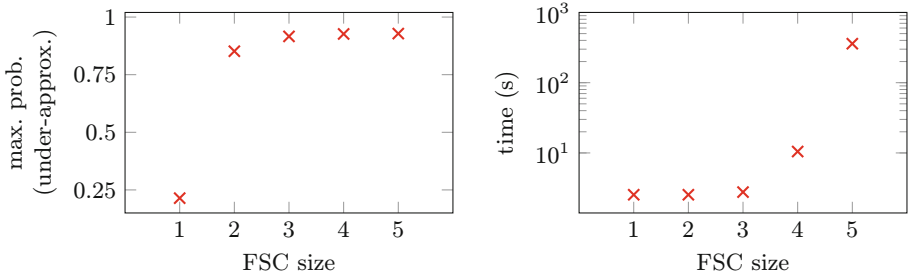
Fig. 5. Max. prob. achieved and time to compute the FSC for grid-avoid with PAYNT
