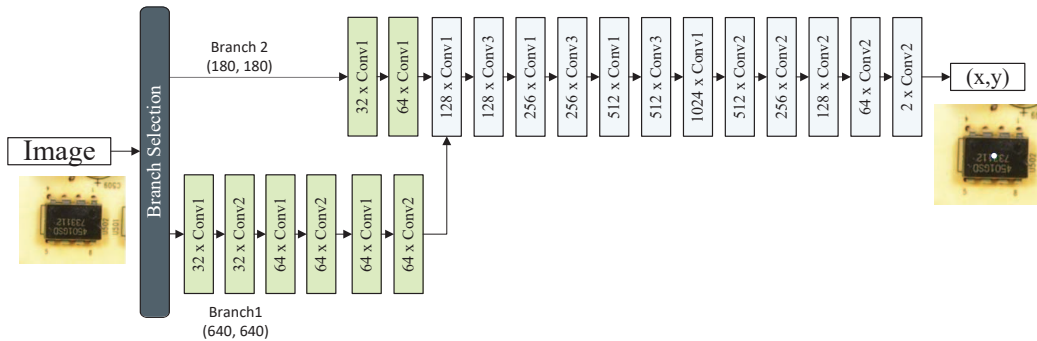
Fig. 5. Case 2: Model with 2 input branches, with input dimensions (640,640) and (180, 180)
