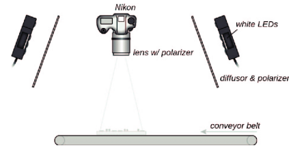
Fig. 7. Data collection setup for PCB-DSLR Dataset [4]
