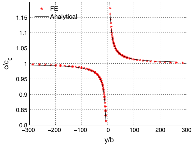
Fig. 4 Variations of the normalised steady-state vacancy concentration profile along y/b at x = 0 , obtained both analytically and numerically
