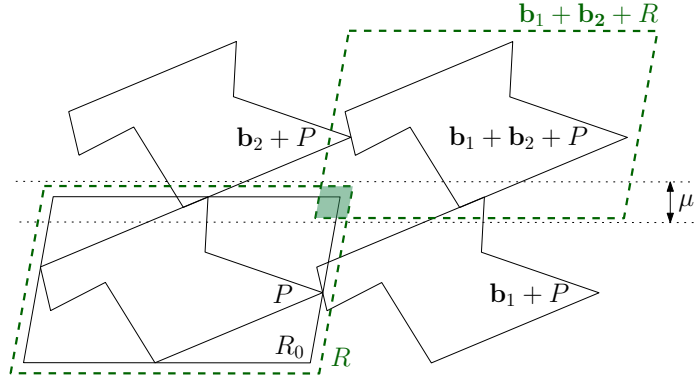
■ Figure 6 Part of the grid k\mathbf{b}_1 + \ell\mathbf{b}_2 + P .
