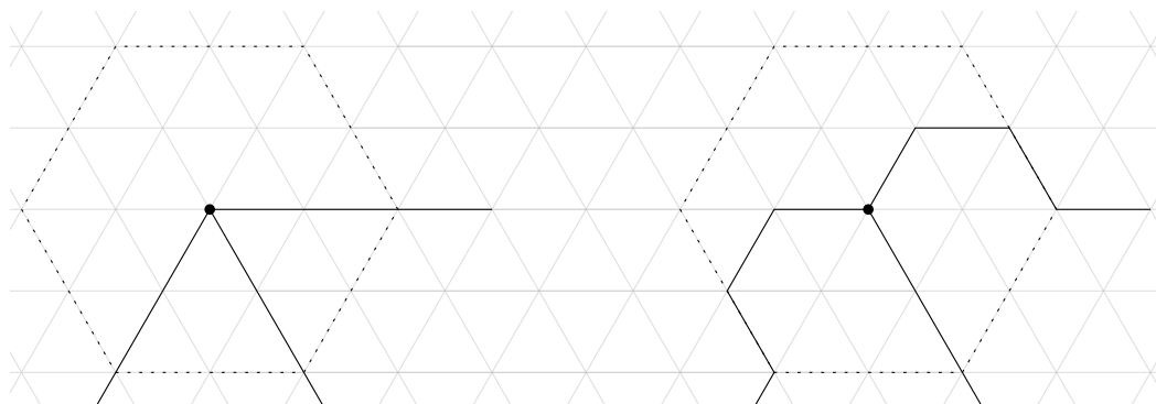
■ Figure 7 Increasing angular resolution in the neighborhood of a vertex
