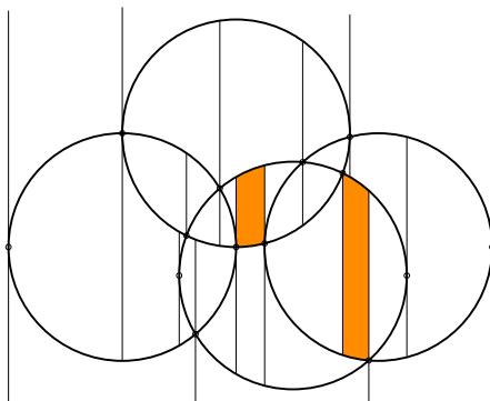
■ Figure 2 Two faces of a vertical decomposition.
