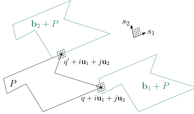
■ Figure 3 A good choice of \mathbf{b}_1, \mathbf{b}_2 and offsets.
