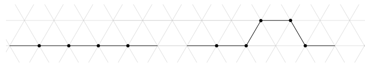
■ Figure 9 Adding a detour to the path of a positive literal
