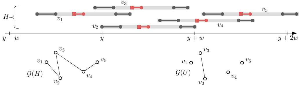
■ Figure 1 Patterns in a window [y - w, y + 2w] . Intervals of U are red.
