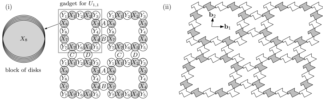
■ Figure 11 (i) The construction by Marx for disks. (ii) Construction with translates of square-like shapes.
