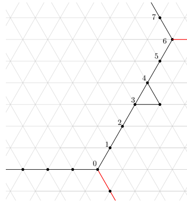
■ Figure 8 Adding an ear to a variable cycle. The black edges are edges of the variable circle, the red edges are on the literal paths.
