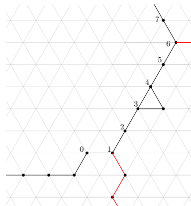
■ Figure 10 Modifying the cycle connection of a negative literal. The black edges are edges of the variable circle, the red edges are on the literal paths.
