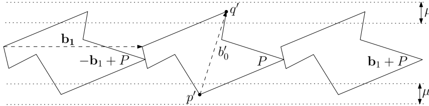
■ Figure 5 Defining \mathbf{b}_2 .
