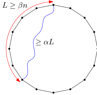
Figure 3: An (\alpha, \beta) -quasi-cycle.
