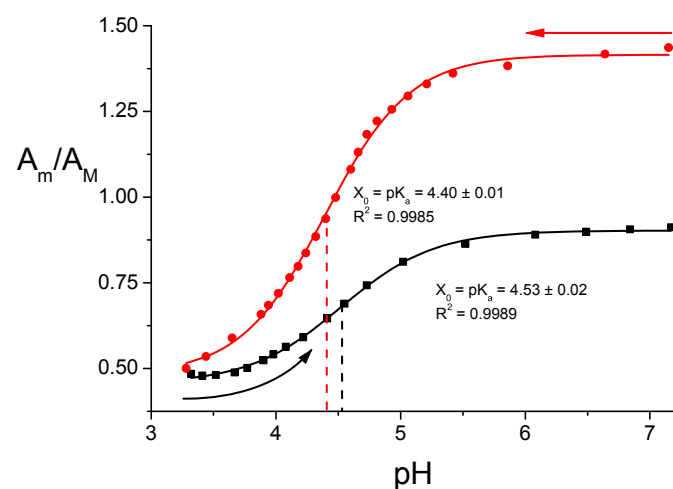
Fig. 1. Displacement of TBO from alginate-TBO stoichiometric complex by \text{H}_3\text{O}^+ (dots) and \text{OH}^- (squares) expressed by the ratio A_m (absorbance metachromatic TBO peak), and A_M (absorbance monomer TBO peak), versus solution pH (in phosphate buffer c = 1 \text{ mM} ). The solid curve represents the fitted sigmoidal functions to both data sets and the centre of the sigmoidal (indicated by the dashed line), X_0 , represents \text{pK}_a ( \text{app} ).
