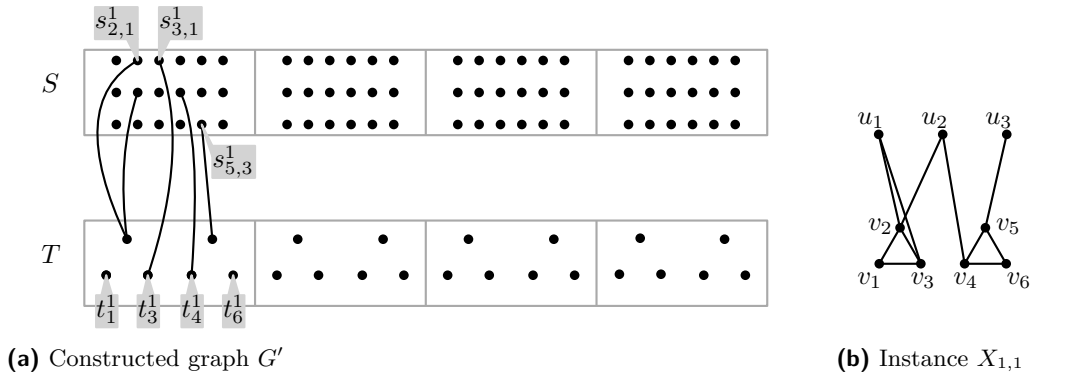
■ Figure 1 Construction of graph G' for t' = 4 , m = 3 , and n = 2 . Edges between vertices in S and T are shown for instance X_{1,1} . All blocking-gadgets and the vertex sets A and B are left out.
