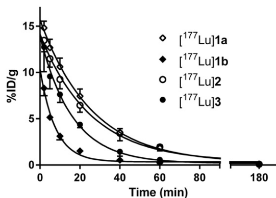
Fig. 4. Blood clearance data of ^{177}\text{Lu} -labeled tetrazines (6.7 nmol, 0.6–1.0 MBq) in non-pretargeted tumor-bearing mice, fitted to a one-phase exponential decay model. Data points represent the % injected dose per gram (%ID/g) and are mean \pm SD ( n = 4 ). For calculated half-lives, see Table 1. The complete raw data are provided in Supplemental Table S6.
