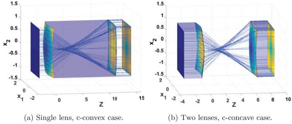
Figure 9: Gaussian to non-uniform distribution: the freeform lens systems.
