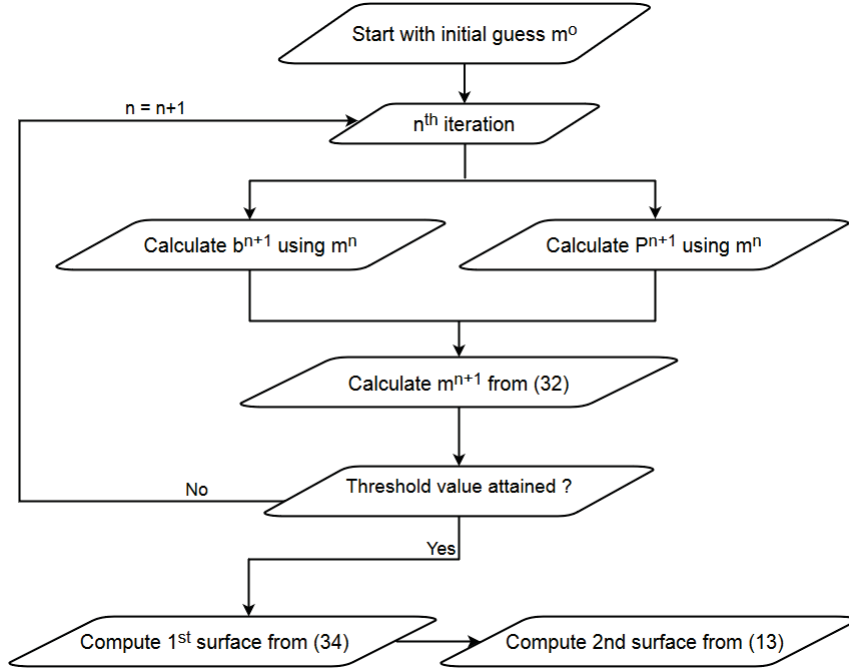
Figure 2: Flow diagram of the proposed algorithm.
