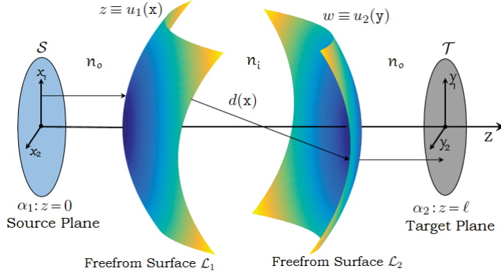
Figure 1: Sketch of a freeform lens optical system
