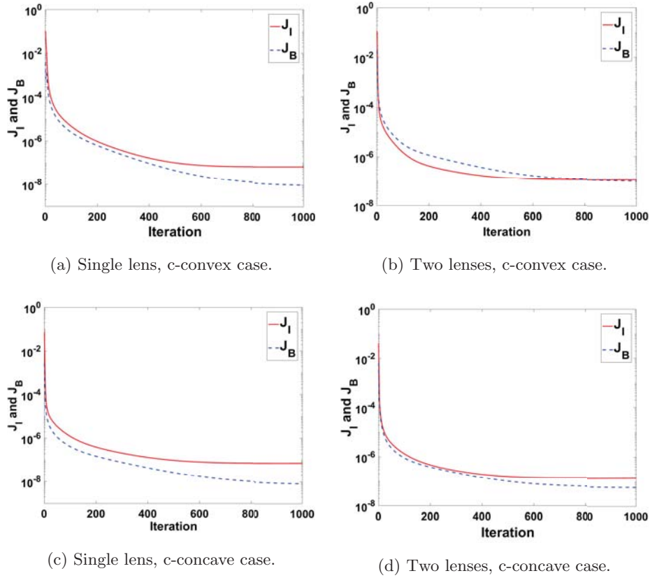
Figure 4: Gaussian to circular top-hat: convergence history of the algorithm.
