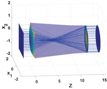
(a) Single lens, c-convex case.
