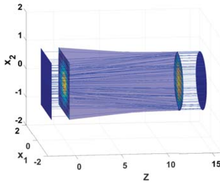
(c) Single lens, c-concave case.
