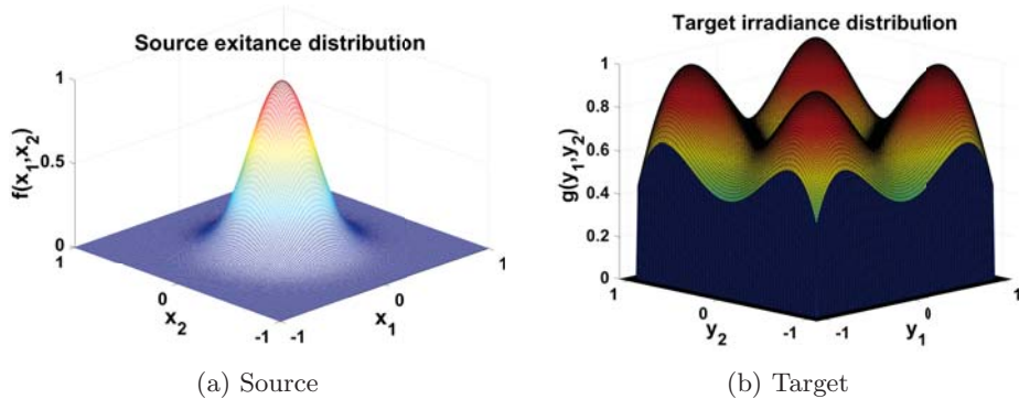
Figure 7: Gaussian to non-uniform: Source and target distributions.
