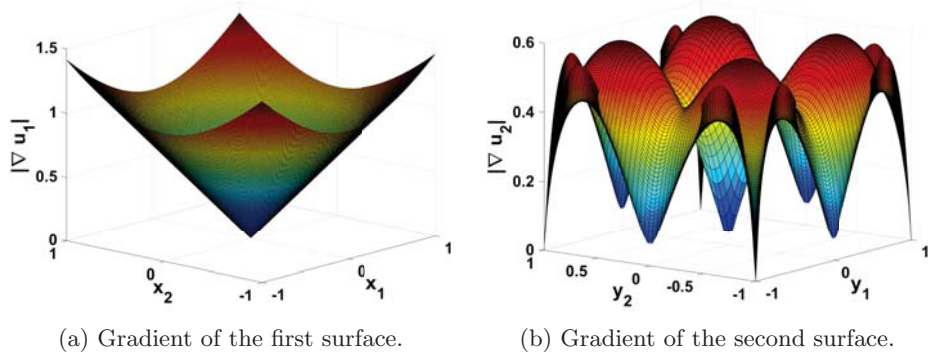
Figure 10: Gaussian to non-uniform distribution, single lens system: modulus of gradients of the freeform surfaces.
