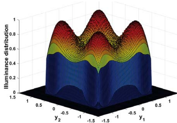
Figure 8: Gaussian-to-non-uniform: Achieved target irradiance distribution.
