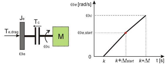
Figure 8: Engine start model.
