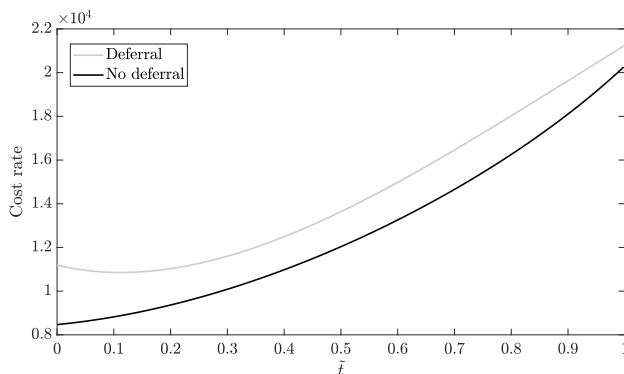
Figure 5: Cost rate in case of deferral and of no deferral for wind industry example. Optimal \tilde{t} is equal to 0.112 and 0 for deferral and no deferral, respectively.
