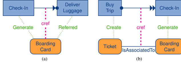
Fig. 6. The two kinds of coreference: (a) over an object class, (b) over a relationship.
