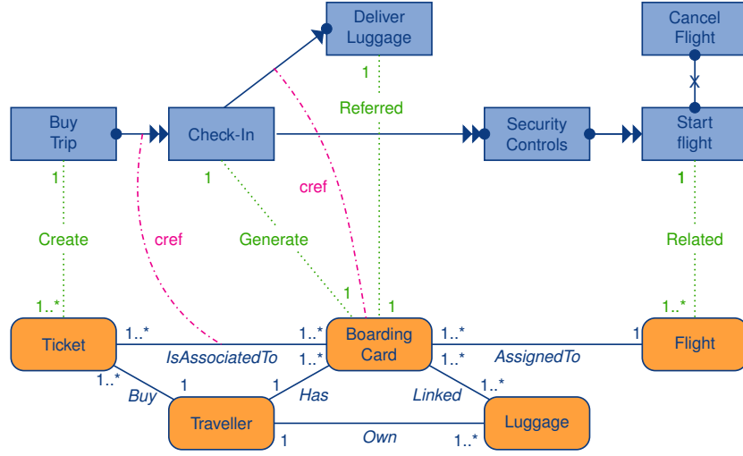
Fig. 5. The OCBCM example of an airplane trip scenario.
