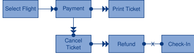
Fig. 4. BCM example capturing the fragment of a ticket purchase process
