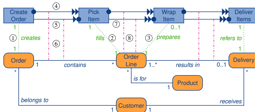
Fig. 1. A small Object-Centric Behavioral Constraint (OCBC) model.
