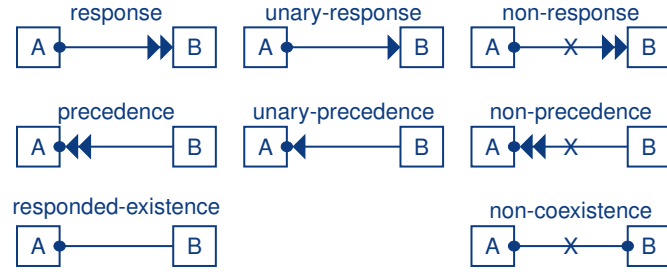
Fig. 2. Types of BCM constraints.
