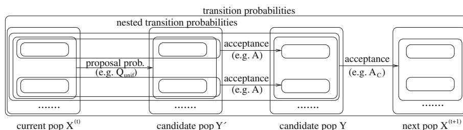
Fig. 1 Nested EMCMC framework: a candidate population \mathbf{Y}' is proposed with some proposal distribution Q from the current population \mathbf{X}' and some children are accepted with some MH
