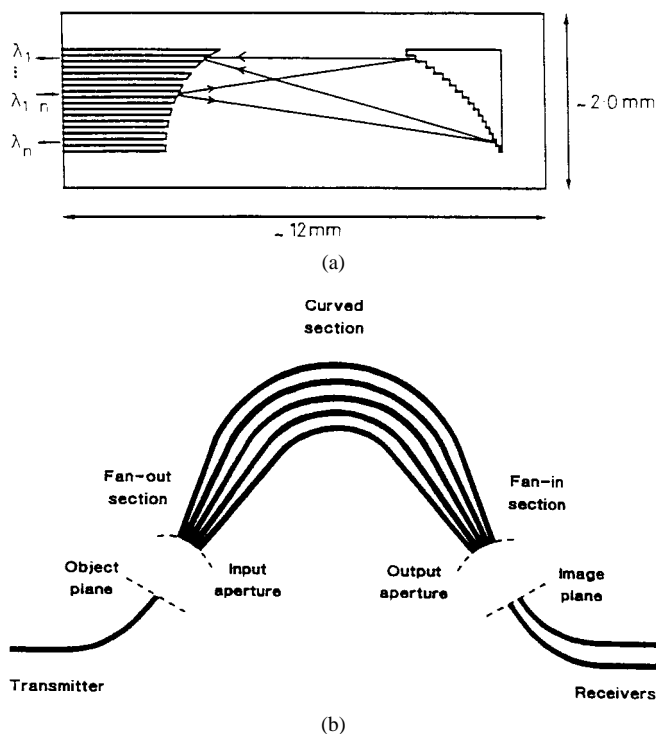
Fig. 15. Two examples of integrated type optical demultiplexers: (a) with a planar reflection grating [66] and (b) with a phased array design [55].
