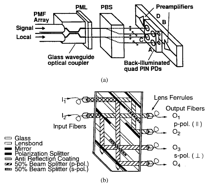
Fig. 9. Examples of diversity optics employing microoptical techniques. The example on top (a) shows a hybrid which contain microoptics and waveguide optics, packaged together with a quad PIN detector [37]. At the bottom, an example is illustrated (b) where critical angle alignments of each expanded beam fiber interface have been avoided owing to a design based on a stack of glass plates with parallel surfaces [46].
