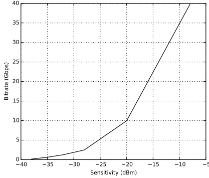
Fig. 6: Bitrate vs receiver sensitivity.
