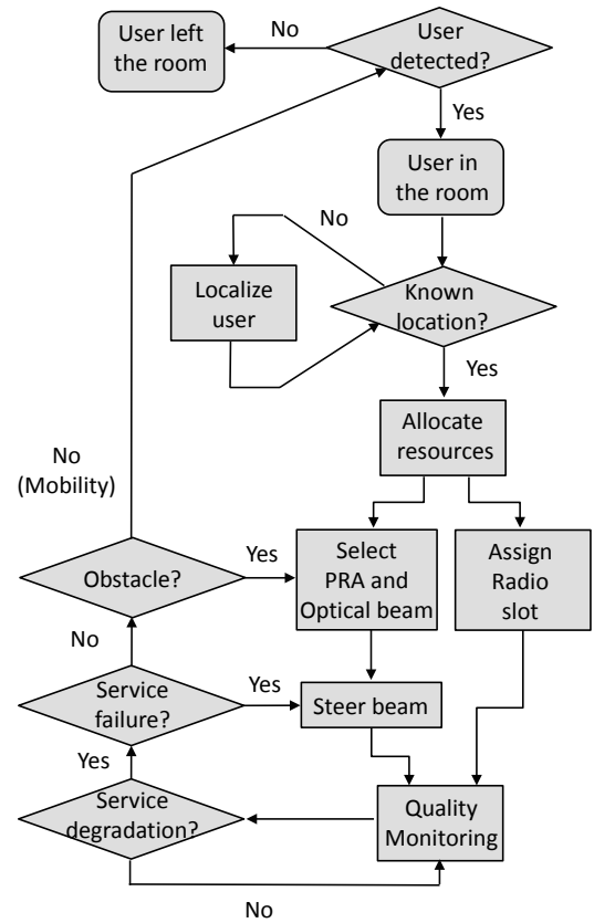
Fig. 2: BROWSE management flow chart.
