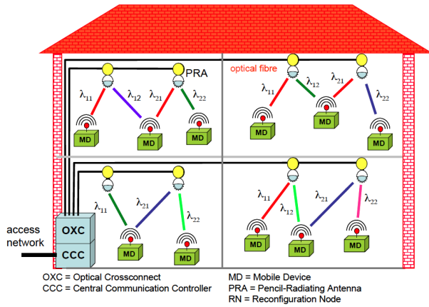
Fig. 1: BROWSE building.
