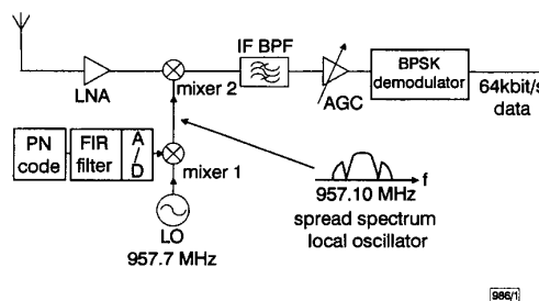
Fig. 1 Interference suppression architecture at direct sequence receiver
