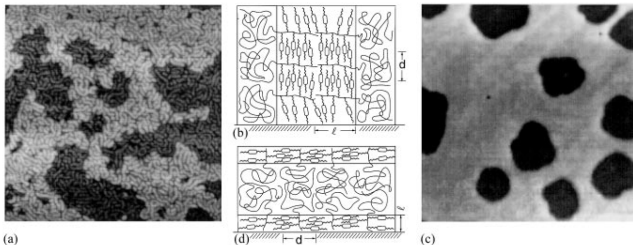
FIG. 2. (a) Perpendicular wetting of the hybrid lamellae in a symmetric ( \Phi_{\text{PS}} = 0.49, M_n = 57\,000 g/mol) PS-PChEMA diblock film, as observed by AFM ( 2.0 \times 2.0 \mu\text{m}^2 viewing area): The in-plane corrugation period is \sim 320 \pm 40 \text{ \AA} , which is essentially L_0 . (b) A schematic representation of perpendicular wetting: Note relative sizes of the smectic spacing d and the interfacial block size \ell : \ell > d and \ell \neq Nd , where N is a positive integer. (c) Generic parallel wetting of the hybrid lamellae in an asymmetric ( \Phi_{\text{PS}} = 0.64, M_n = 36\,000 g/mol) diblock film, as observed by AFM ( 4.0 \times 4.0 \mu\text{m}^2 viewing area): The height difference between the two domains is \sim 150 \pm 15 \text{ \AA} , which is equal to L_0 for this diblock. (d) A schematic representation of parallel wetting: d > \ell .
