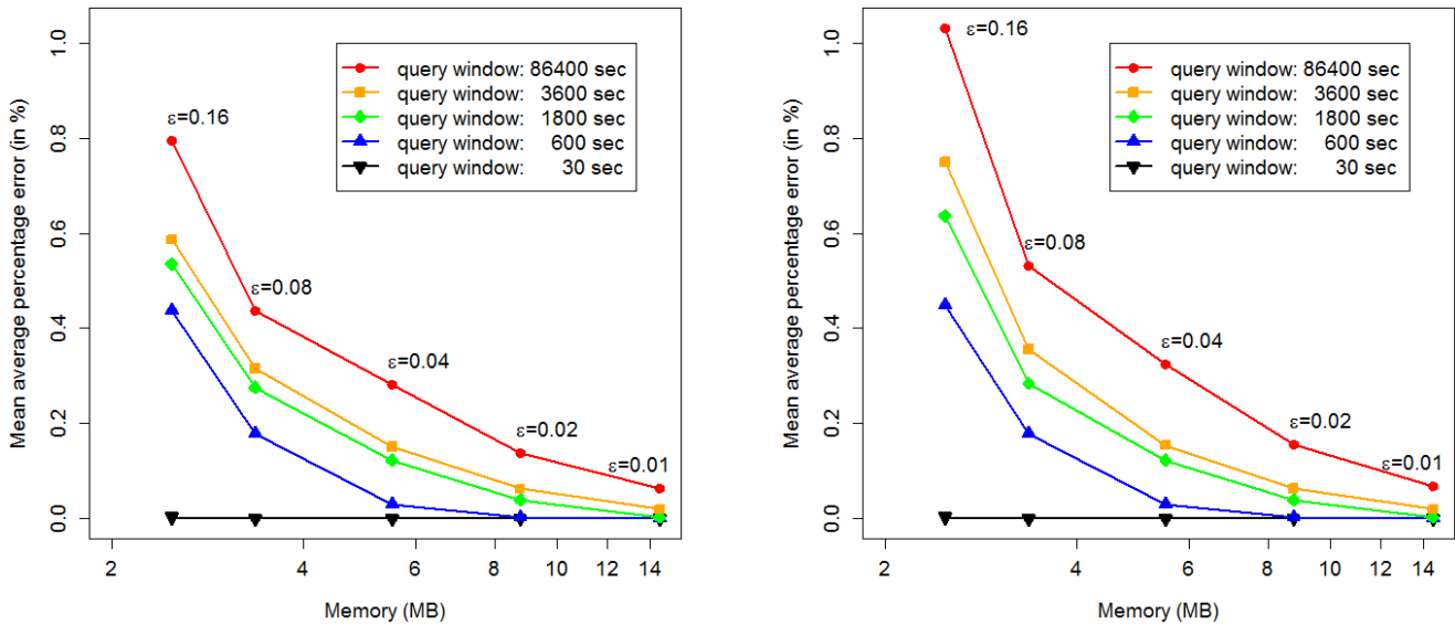
Figure 3: Mean average percentage error and memory usage for different maximum relative errors ( \varepsilon ) and query window sizes; left: without intermediate nodes; right: hierarchy with 10 intermediate nodes
