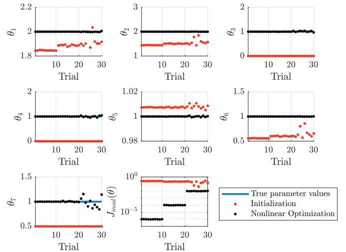
Fig. 3. Simulation results for different noise intensities. The first 10 trials correspond to \sigma_e^2 = 10^{-6} , the second 10 to \sigma_e^2 = 10^{-4} and the last 10 to \sigma_e^2 = 10^{-2} .
