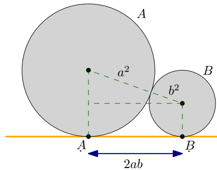
Figure 3: The footprint distance of two touching disks.
