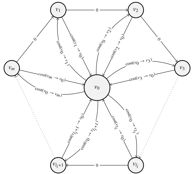
Fig. 6. Directed graph G in Section 5.2.1.
