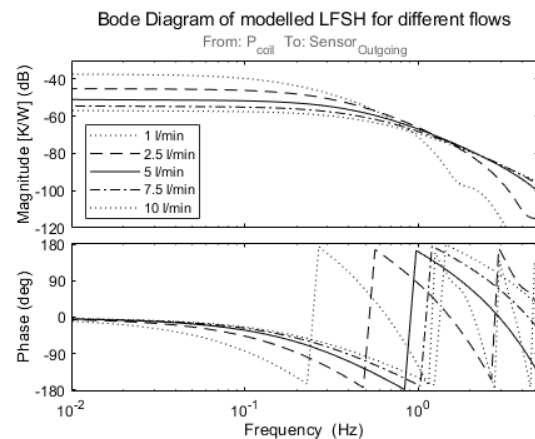
Figure 2. Frequency response from the coil power to the outgoing water temperature of the LFSH for multiple flow rates.
