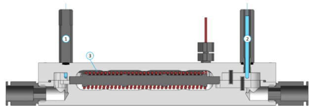
Figure 1. A cross-section of the Local Fluid Stream Heater used in this research, with incoming temperature sensor (1), outgoing temperature sensor (2) and heater coil (3).
