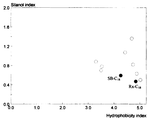
Fig. 4. Scatter plot of silanol index versus hydrophobicity index of several commercially available C 18 RP-HPLC column materials according to Walters.
