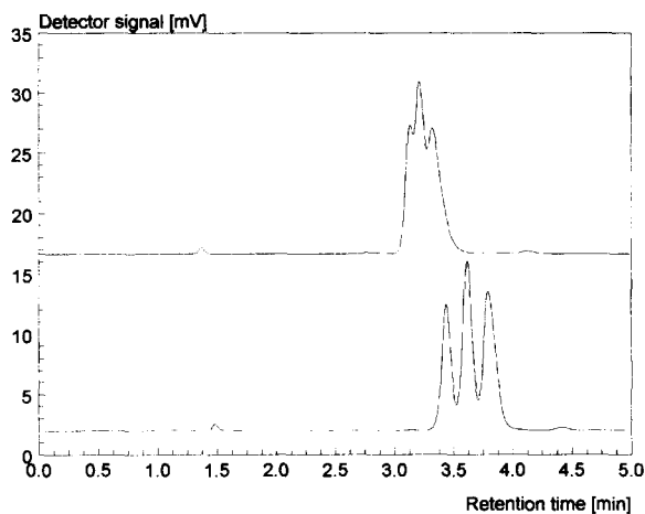
Fig. 2. Chromatograms of the toluidine isomers (elution order: ortho -, meta -, para -toluidine) on a Rx-C 18 column (upper trace) and on a SB-C 18 column (lower trace). Eluent: MeOH–H 2 O (55:45, v/v). Flow-rate: 1.0 ml/min. Injected amount: 0.3 µg per component.
