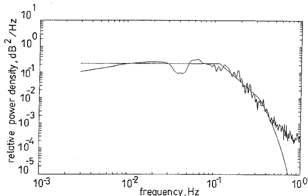
Fig. 4 Theoretical and experimental power spectral density function of amplitude scintillation measured on 12.5GHz beacon signal of Olympus satellite at EUT ground station 13th June 1992, 12.00 – 12.23h GMT
