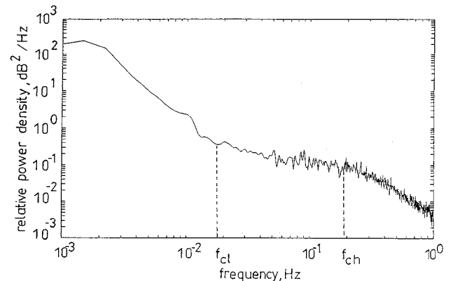
Fig. 1 Power spectral density function of event with concurrent rain attenuation and amplitude scintillation measured on 30 GHz beacon signal of Olympus satellite at EUT ground station 8th August 1992, 01.00 – 04.48h GMT
