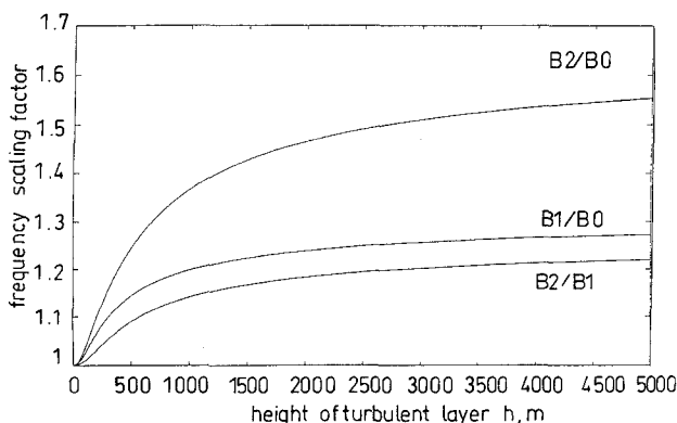
Fig. 2 Frequency scaling factor as function of height of turbulent layer n = 11/3 , \sqrt{\eta_{B0}} = \sqrt{\eta_{B1}} = \sqrt{\eta_{B2}} = 0.75
