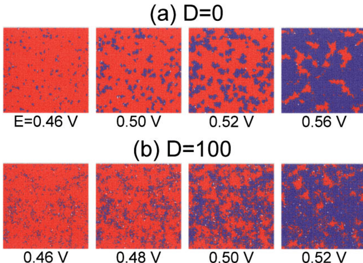
FIG. 9. Snapshots of the electrode surface during the voltammograms of Fig. 8(a). Blue, OH; Red, CO; White, empty site.
