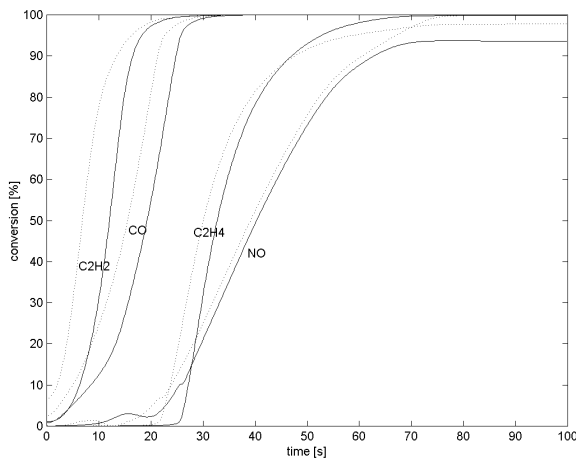
Figure 4. Conversions after a step increase of the feed temperature from 400 to 500K. Solid lines – ethyne forms 30% of hydrocarbons; dashed lines – ethyne forms 10% of hydrocarbons.
