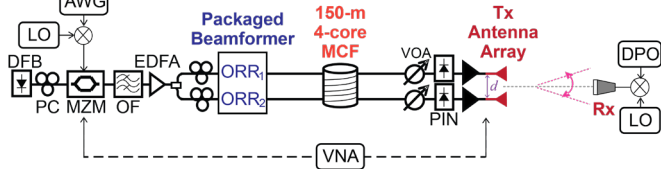
Figure 4. Experimental set-up of an optical beamformer controlling a 1 \times 2 antenna array employing MCF.
