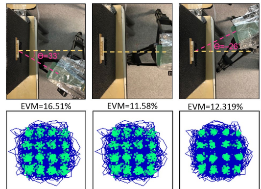
Figure 7. Measured EVM after wireless transmission of 1.5 GHz-BW 16QAM-modulated signals at 33^\circ , 0^\circ , and -26^\circ steering angles.
