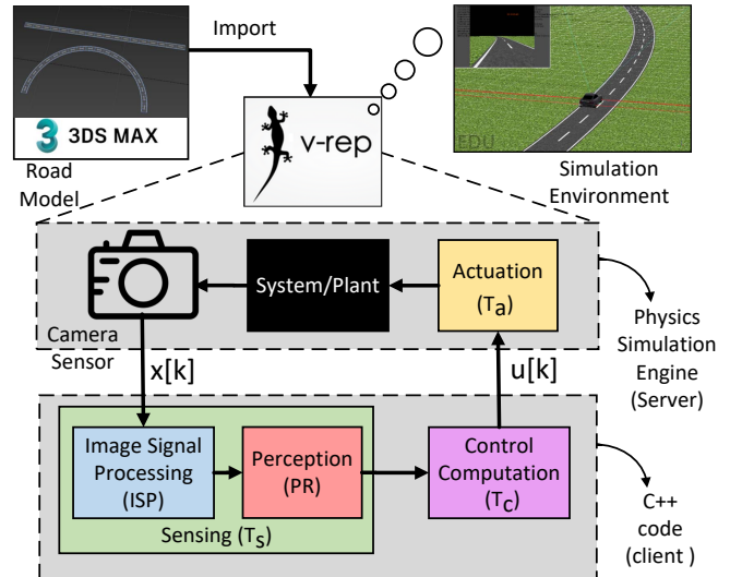
Fig. 2. SiL simulator setup for LKAS system.
