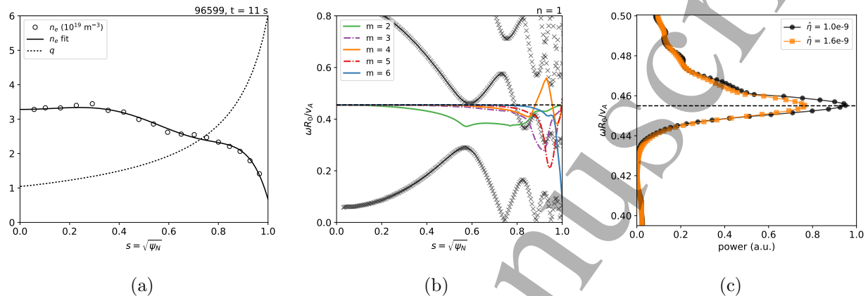
Figure 9: (a) Density and safety factor profiles for JPN 96599 at t = 11 s (limiter configuration). (b) Alfvén continua (crosses) from CSCAS overlaid with the real part of velocity perturbation (solid, dot-dashed) from CASTOR for n = 1 , m = 2 to 6 , and eigenvalue \omega_0 R_0/v_A = 0.455 (dashed). (c) Power absorbed versus frequency from CASTOR for two normalized resistivities \hat{\eta} = 1.0 \times 10^{-9} and 1.6 \times 10^{-9} . Note the different horizontal and vertical axes.
