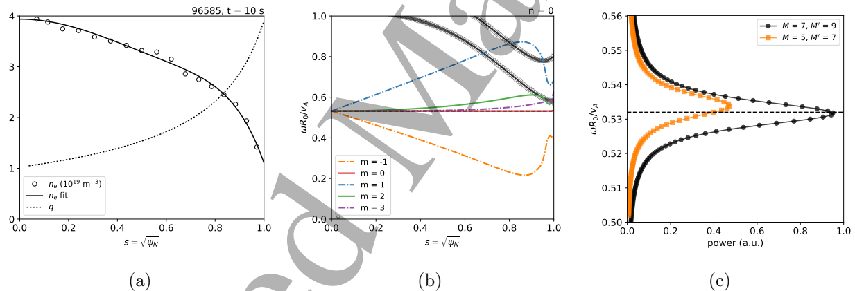
Figure 4: (a) Density and safety factor profiles for JPN 96585 at t = 10 s. (b) Alfvén continua (crosses) from CSCAS overlaid with the real part of velocity perturbation (solid, dot-dashed) from CASTOR for n = 0 , m = -1 to 3, and eigenvalue \omega_0 R_0/v_A = 0.532 (dashed). (c) Power absorbed versus frequency from CASTOR for two simulation “domain” sizes, with M and M' the number of poloidal harmonics of the plasma/antenna and of the vacuum, respectively. Note the different horizontal and vertical axes.
