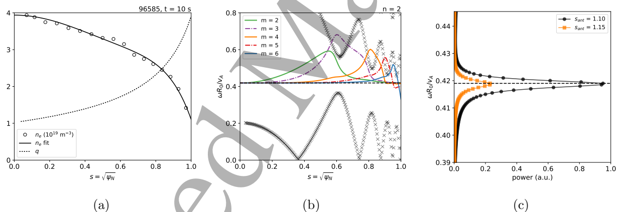
Figure 5: (a) Density and safety factor profiles for JPN 96585 at t = 10 s (same as Fig. 4a). (b) Alfvén continua (crosses) from CSCAS overlaid with the real part of velocity perturbation (solid, dot-dashed) from CASTOR for n = 2 , m = 2 to 6, and eigenvalue \omega_0 R_0/v_A = 0.419 (dashed). (c) Power absorbed versus frequency from CASTOR for two plasma-antenna separations, with antenna radial positions s_{\text{ant}} = 1.10 and 1.15. Note the different horizontal and vertical axes.
