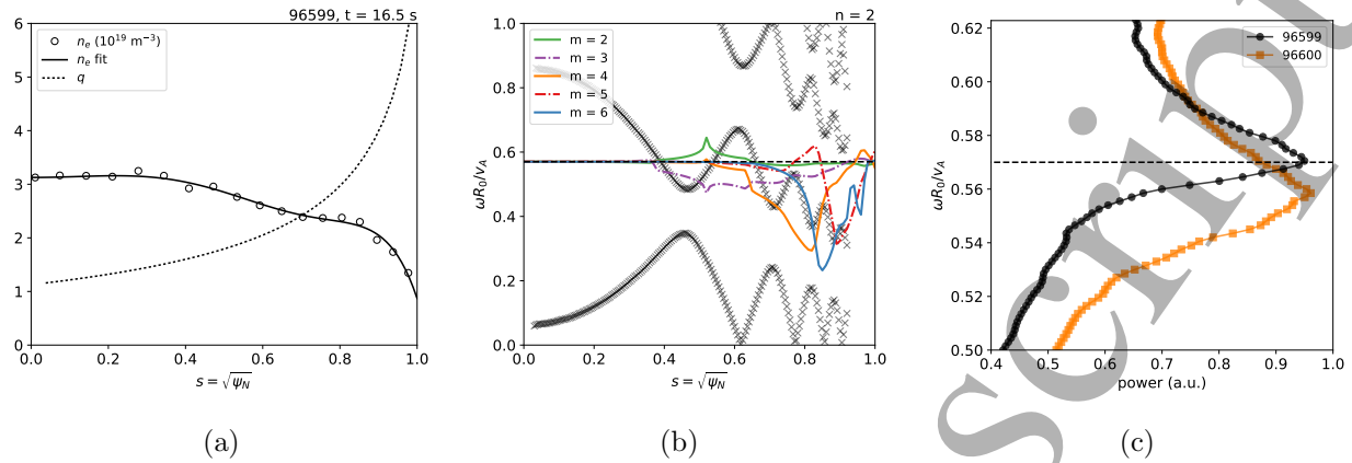
Figure 10: (a) Density and safety factor profiles for JPN 96599 at t = 16.5 \text{ s} (X-point configuration). (b) Alfvén continua (crosses) from CSCAS overlaid with the real part of velocity perturbation (solid, dot-dashed) from CASTOR for n = 2 , m = 2 to 6, and eigenvalue \omega_0 R_0/v_A = 0.570 (dashed). (c) Power absorbed versus frequency from CASTOR for JPN 96599 and 96600 (also at t = 16.5 \text{ s} ). Note the different horizontal and vertical axes and limits.
