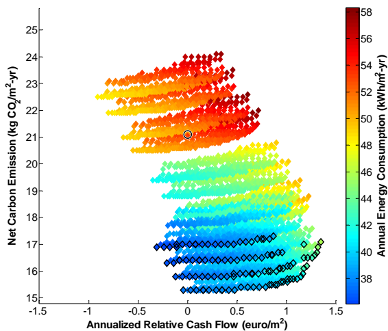
Figure 5 Pareto solutions of Scenario 3
