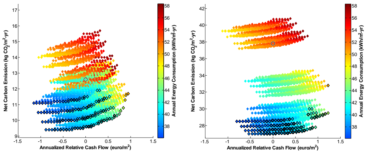
Figure 4 Design solutions of Scenario 1 and 2
