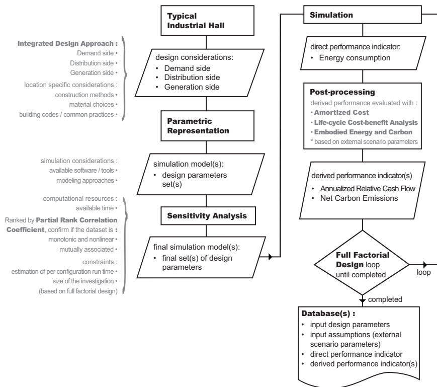
Figure 1 Flowchart of the design support with the full-factorial design space exploration approach
