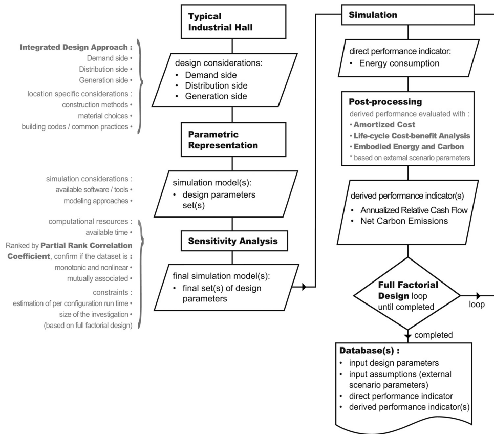
Fig. 1. Flowchart of the design support with the full-factorial design space exploration approach.
