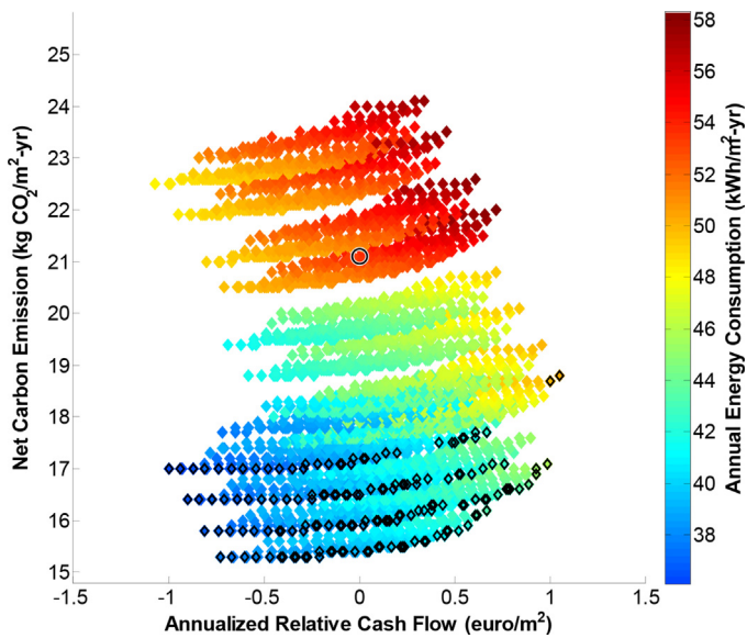
Fig. 3. Pareto solutions (shown with black outline) with respect to three design objectives among all studied configurations (color diamonds). (For interpretation of the references to color in this figure legend, the reader is referred to the web version of this article.)
