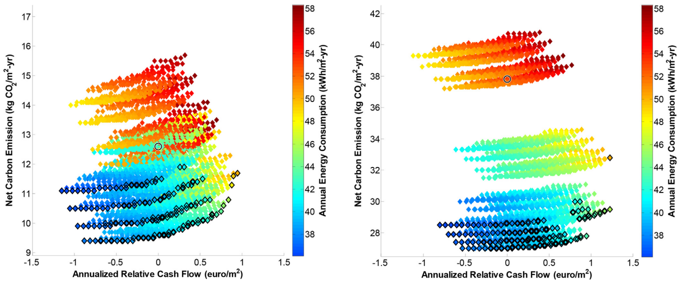
Fig. 4. Design solutions of Scenario 1 and 2.
