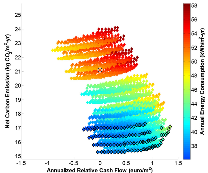
Fig. 5. Pareto solutions of Scenario 3.
