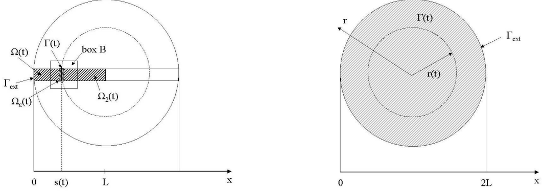
Figure 3: On the left: Fig. 3a, on the right Fig. 3b. Cross sections of concrete samples. The modeling area \Omega is a rectangle or an interval, respectively. Interactions with the parts on top and below the bottom of \Omega are neglected, vertical changes are considered as constant. The whole setting is 1D . On the right: The whole cross section of the sample is the modeling area \Omega , i.e. the setting is 2D .
