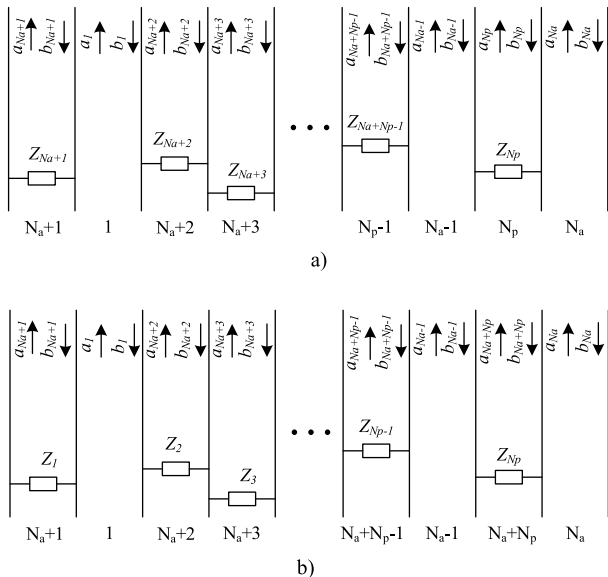
Fig. 1. Schematic of a reactively loaded antenna array. (a) Original illustration. (b) Corrected illustration.
