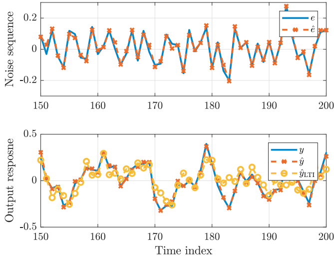
Fig. 2. Top: True innovation noise sequence e and estimated innovation noise sequence \hat{e} . Bottom: True response y , response \hat{y} of nonlinear model \mathcal{M}_{\hat{e}} and response \hat{y}_{LTI} of the identified LTI model.
