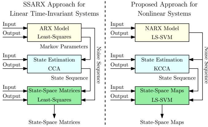
Fig. 1. Existing SSARX approach for LTI system (left). Proposed identification approach for nonlinear systems (right).
