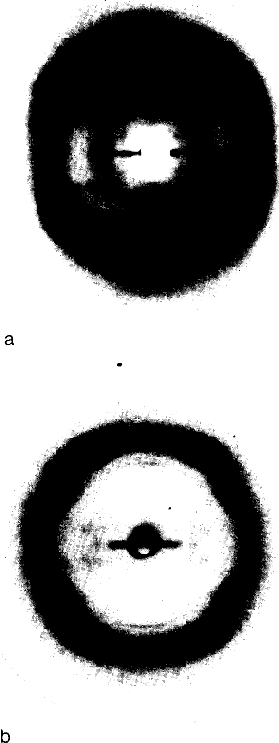
Figure 2 X-ray fibre diffraction patterns of i-PS gels: (a) i-PS in trans -decalin showing rather weak odd order layer lines at spacing 3.06 nm; (b) i-PS in cis -decalin showing strong first order layer line, again with spacing 3.06 nm
