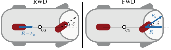
Fig. 2. Traction force for RWD and FWD configurations.
