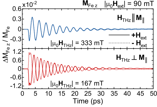
FIG. 3. Dynamics of the z component of iron M_{\text{Fe}} modeled by Landau-Lifshitz-Gilbert equations. Note that at high THz fluences and low temperatures, the blue curves for two field polarities are not exactly symmetric, as can be seen in Fig. 1 (b). A possible reason for this behavior could be an onset of higher-order effects in the detection of spins such as the magneto-optical Cotton-Mouton effect.
