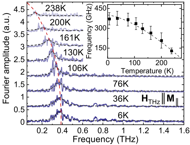
FIG. 2. Fourier spectrum of the THz-induced signal ( \mathbf{H}_{\text{THz}} \parallel \mathbf{M}_{\parallel} ) measured at various temperatures. Central frequencies of the peaks deduced from the fit are plotted as a function of temperature in the inset. The dotted line denotes a fit with Eq. (8) ( \omega_0/2\pi = 400 GHz, T_C = 314 K) and the bars denote \pm half-width-half-maximum of the fitted Lorentzians. The fast Fourier transform spectrum for \mathbf{H}_{\text{THz}} \perp \mathbf{M} is added to the Supplemental Material (Fig. S8) [17].
