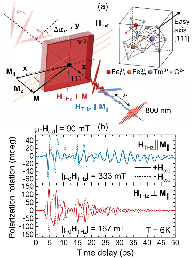
FIG. 1. (a) Schematic of the experimental setup. The illustration on the top right shows the distribution of dodecahedral \text{Tm}^{3+} and tetrahedral/octahedral \text{Fe}^{3+} ions. Any magnetic moment will tend to align along the [111] “easy axis.” (b) Polarization rotation \Delta\alpha_F measured as a function of the time delay \tau between THz pump and optical probe pulses. Depending on the THz polarization, the mapped dynamics is either odd ( \mathbf{H}_{\text{THz}} \parallel \mathbf{y} \perp \mathbf{M}_{\parallel} ) with the external magnetic field or even ( \mathbf{H}_{\text{THz}} \parallel \mathbf{x} \parallel \mathbf{M}_{\parallel} ). The measurements were performed at T = 6 K.
