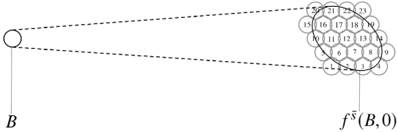
Fig. 3. Alphabet for the ball B_\delta of Fig. 2
