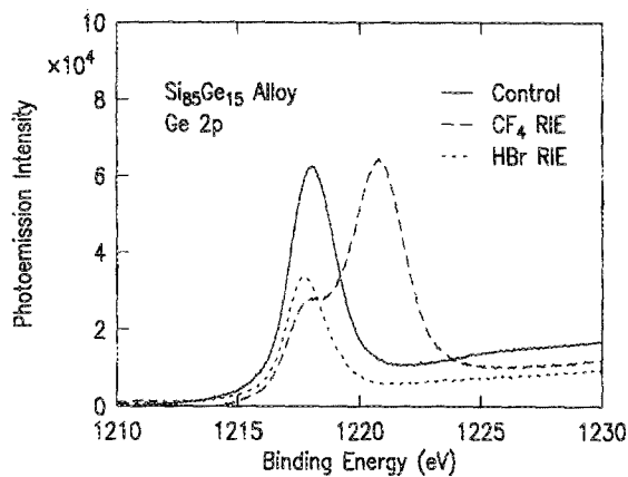
FIG. 5. Ge 2p_{3/2} photoelectron spectra of epitaxial SiGe film (15% Ge) control and after reactive ion etching using CF_4 and HBr (see Fig. 4).
