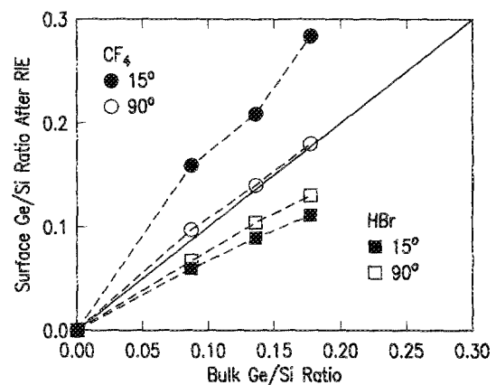
FIG. 6. The surface Ge/Si element ratio of SiGe alloys after CF_4 and HBr RIE as obtained by Ge 3p and Si 2p photoemission as a function of the bulk Ge/Si ratio of the alloy obtained by Rutherford backscattering spectrometry.
