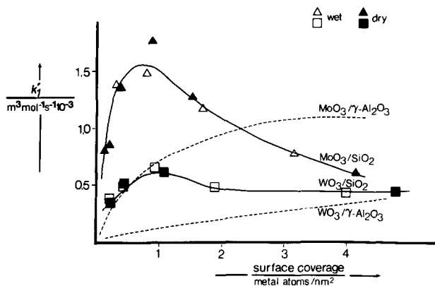
FIG. 3. Reaction rate constant k_1' for the hydrodesulfurization of thiophene as a function of the average surface coverage for sulfided MoO 3 /SiO 2 , WO 3 /SiO 2 , MoO 3 /γ-Al 2 O 3 , and WO 3 /γ-Al 2 O 3 catalysts prepared by dry and wet impregnation (data for alumina-based catalysts are presented in Ref. (1)).
