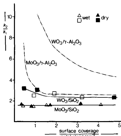
FIG. 5. Ratio between reaction rate constants from the hydrogenation of butene and the hydrodesulfurization of thiophene, k_2/k_1 , as a function of the average surface coverage, for sulfided MoO 3 /SiO 2 , WO 3 /SiO 2 , MoO 3 /γ-Al 2 O 3 , and WO 3 /γ-Al 2 O 3 catalysts, prepared by dry and wet impregnation (data for alumina-based catalysts are presented in Ref. (1)).
