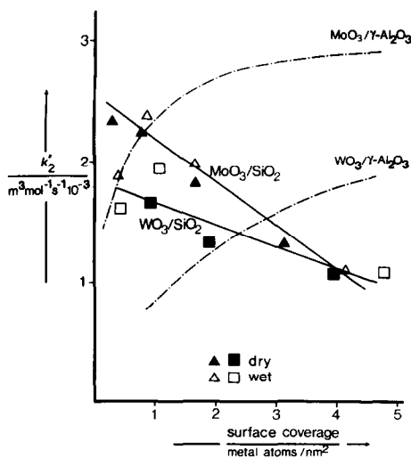
FIG. 4. Reaction rate constant k_2' for the hydrogenation of butene as a function of the average surface coverage for sulfided MoO 3 /SiO 2 , WO 3 /SiO 2 , MoO 3 /γ-Al 2 O 3 , and WO 3 /γ-Al 2 O 3 catalysts prepared by dry and wet impregnation (data for alumina-based catalysts are presented in Ref. (1)).
