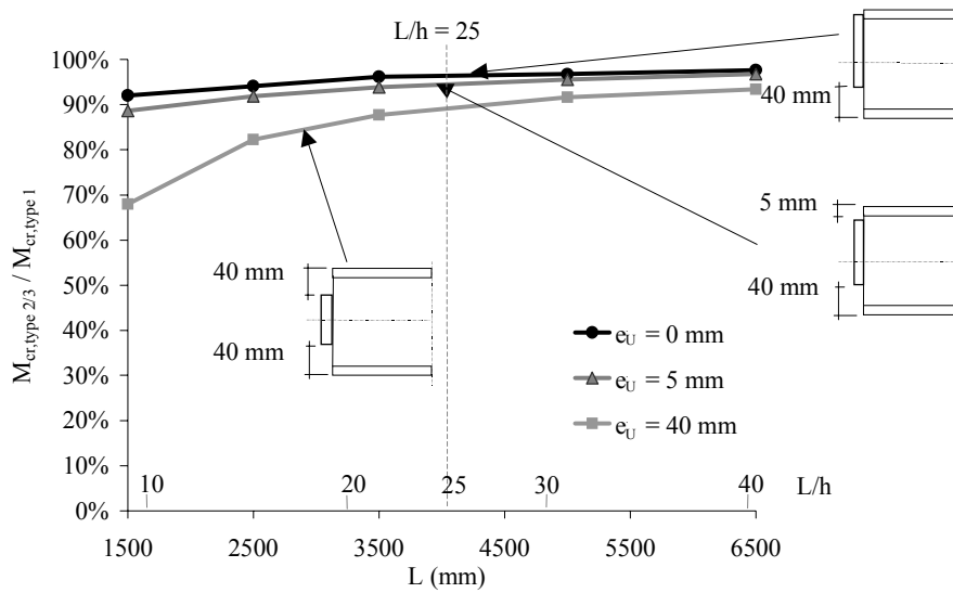
Figure 18: Endplate influence on critical load as a function of span on IPE160 beams
