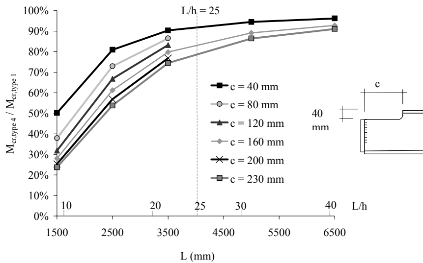
Figure 22: Reduction in critical load due to cope length for beams with type 4 connections with various spans
