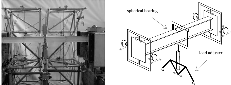
Figure 35: Test set-up
