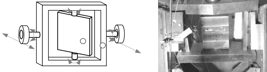
Figure 36: Cardan supports
