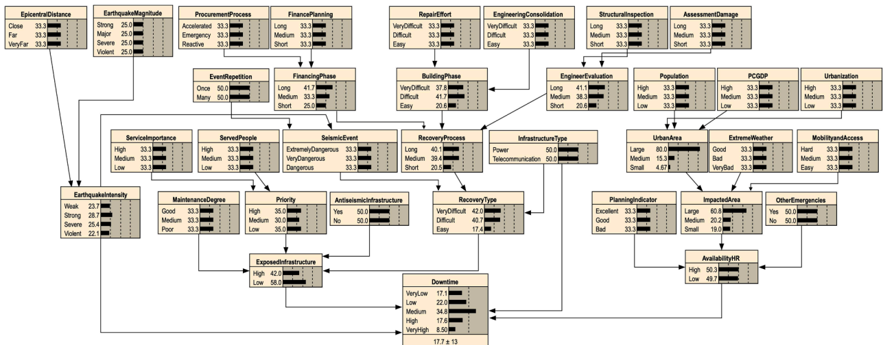
Fig. 8. The Bayesian network of the Downtime indicators using Netica software.
