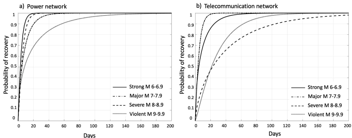
Fig. 5. Restoration curves of (a) the power infrastructure, and (b) the telecommunication infrastructure based on earthquake magnitude.
