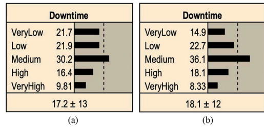
Fig. 11. Downtime evaluation for a) Power network and b) Telecommunication system for Scenario 3.
