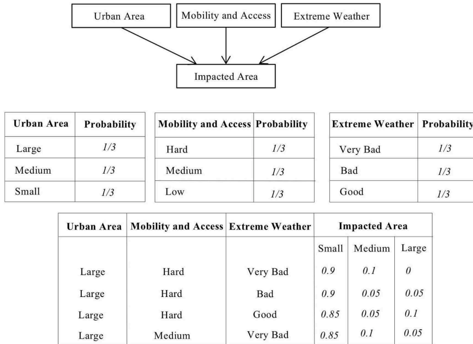
Fig. 2. A three-node network with probability tables.
