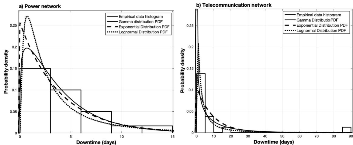
Fig. 4. Histograms and PDF fitting distributions for (a) the power infrastructure, and (b) the telecommunication infrastructure for the data related to earthquake magnitude range M6-6.9.
