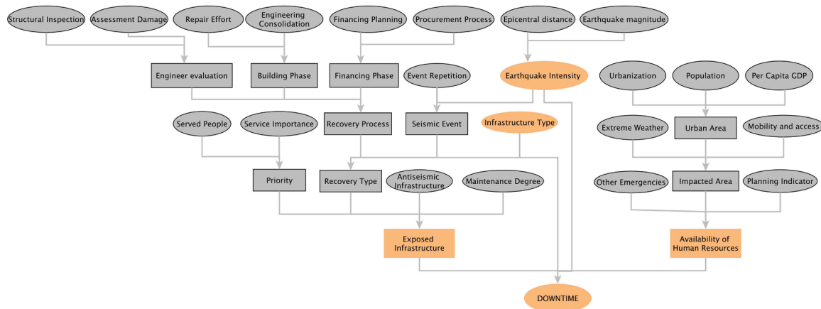
Fig. 3. Downtime assessment model for power and telecommunication infrastructures.
