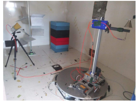
Fig. 2. RC setup to measure G_{\text{ref}} for eight absorbers. The chamber contains one vertical paddle for mode stirring, a turntable with height translation for position stirring, and automated polarization stirring.
