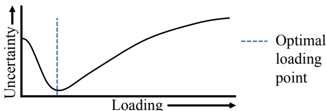
Fig. 5. Illustration of the expected effect on uncertainty by an increase in chamber loading. Uncertainty first decreases because there are more significant modes in the channel bandwidth, but increases for higher loading due to high correlations.
