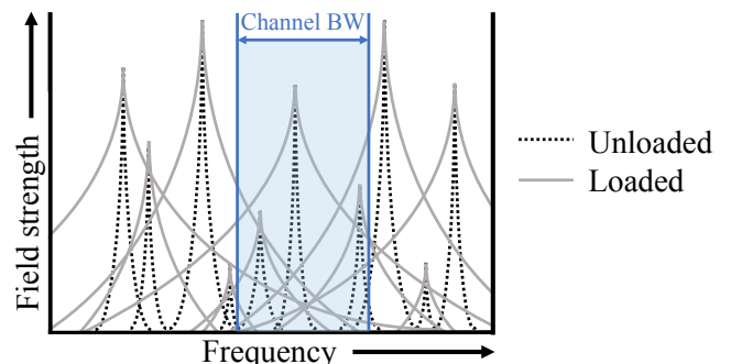
Fig. 4. Illustration of the mode distribution in a loaded and an unloaded RC. The modes spread more across frequency in the channel bandwidth for higher loading cases. Even though these are all correlated within the CBW, sharp peaks and nulls are flattened by the addition of more significant modes.
